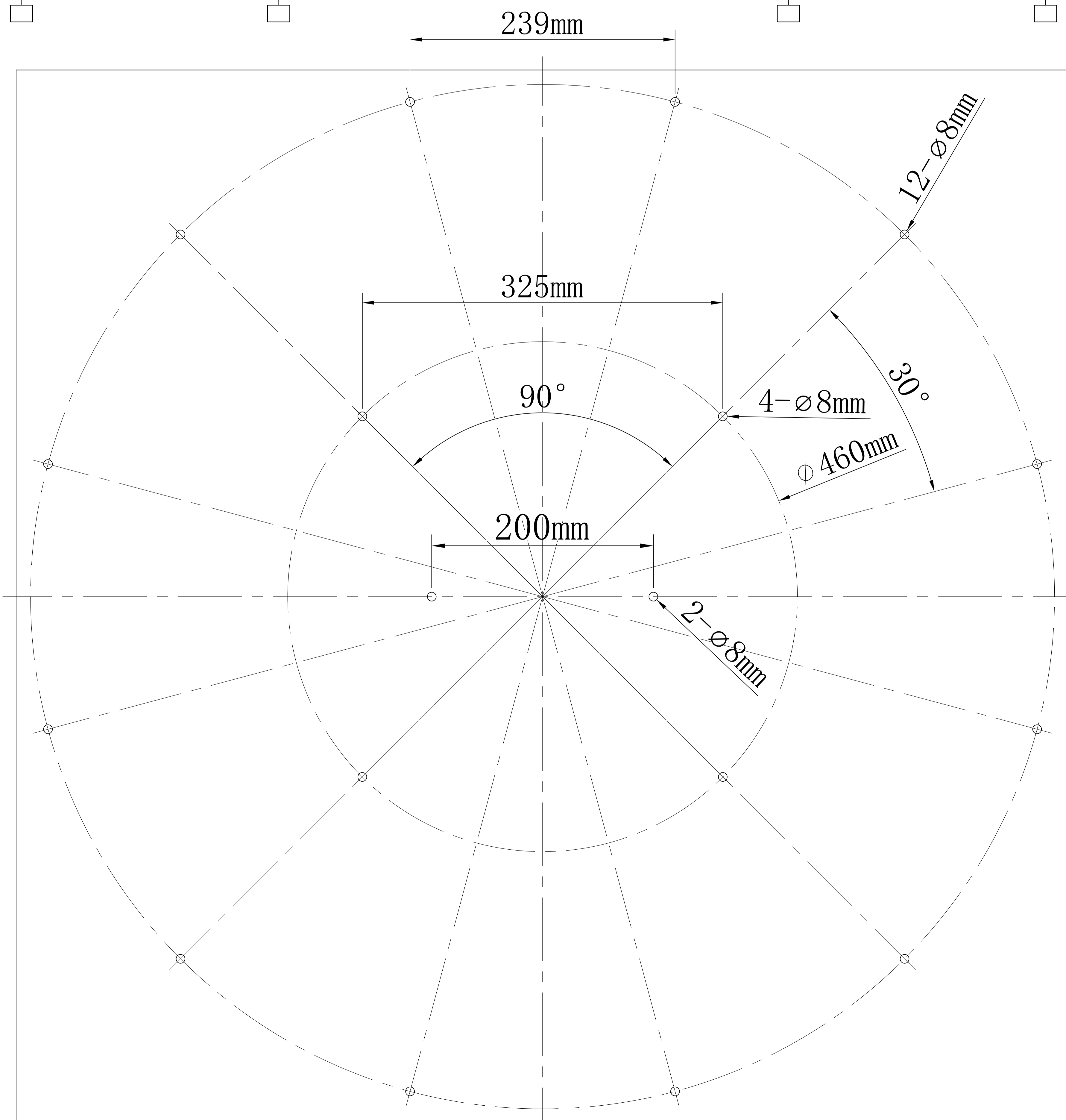
THE POSITIONS OF ALL THREAD ROD
